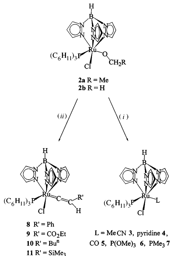
Scheme 2 (i) L; (ii) \text{HC}=\text{CR}'
