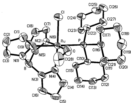
Fig. 1 Structural view of [\text{Ru}\{\text{HB}(\text{pz})_3\}\{\text{P}(\text{C}_6\text{H}_{11})_3\}\text{Cl}(\text{OMe})] 2b . Selected bond lengths (Å) and angles (°): Ru–O 1.943(1), Ru–N(2) 2.133(2), Ru–N(4) 2.084(2), Ru–N(6) 2.109(2), Ru–P 2.394(1) and O–C(28) 1.370(4); C(28)–O–Ru 123.8(2), Cl–Ru–N(4) 174.7(1), N(6)–Ru–O 175.4(1) and N(2)–Ru–P 177.3(1)
